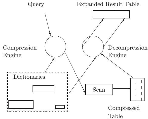
Fig. 4. Querying a database in the compressed form
